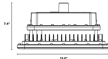
150W - 200W
