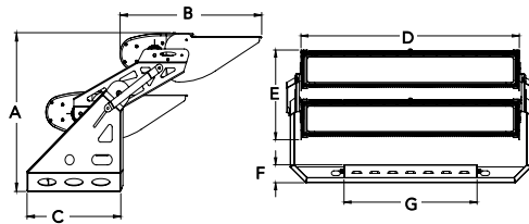
2450W: Trunnion Mounted Driver
