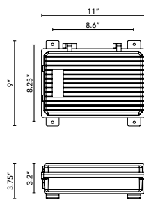
Remote Driver Box B
