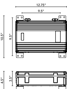
Remote Driver Box A
