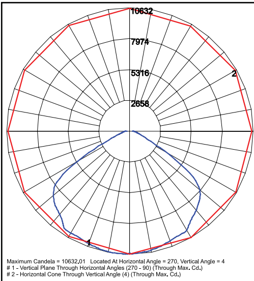
BLD8QW1X200U4K Grid in feet, Mounting Height = 25 ft.
