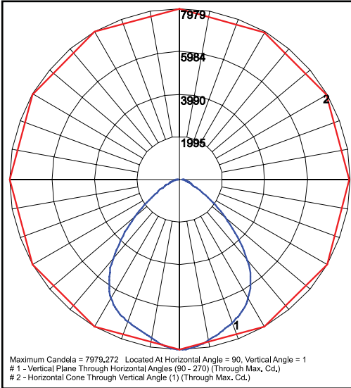
BLD4QW1X100U4K Grid in feet, Mounting Height = 25 ft.
