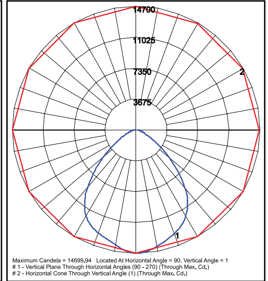
BLD8QW1X200U4K Grid in feet, Mounting Height = 25 ft.
